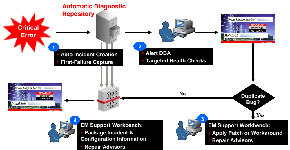
Figure 3: Support workbench workflow
