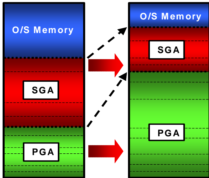
Figure 1: Automatic Memory Management
